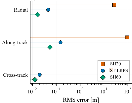
(a) Median
